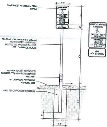
HANDICAP SIGNAGE NOT TO SCALE
