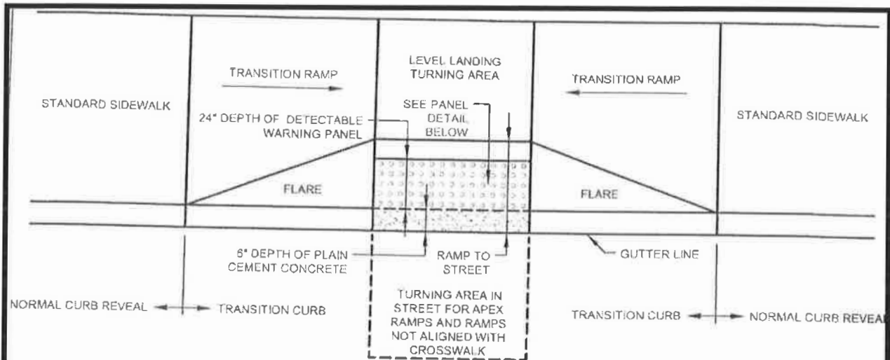
TYPICAL INSTALLATION
