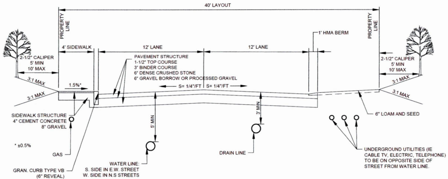
TYPICAL CROSS SECTION - MINOR STREET w/o GRASS STRIP
