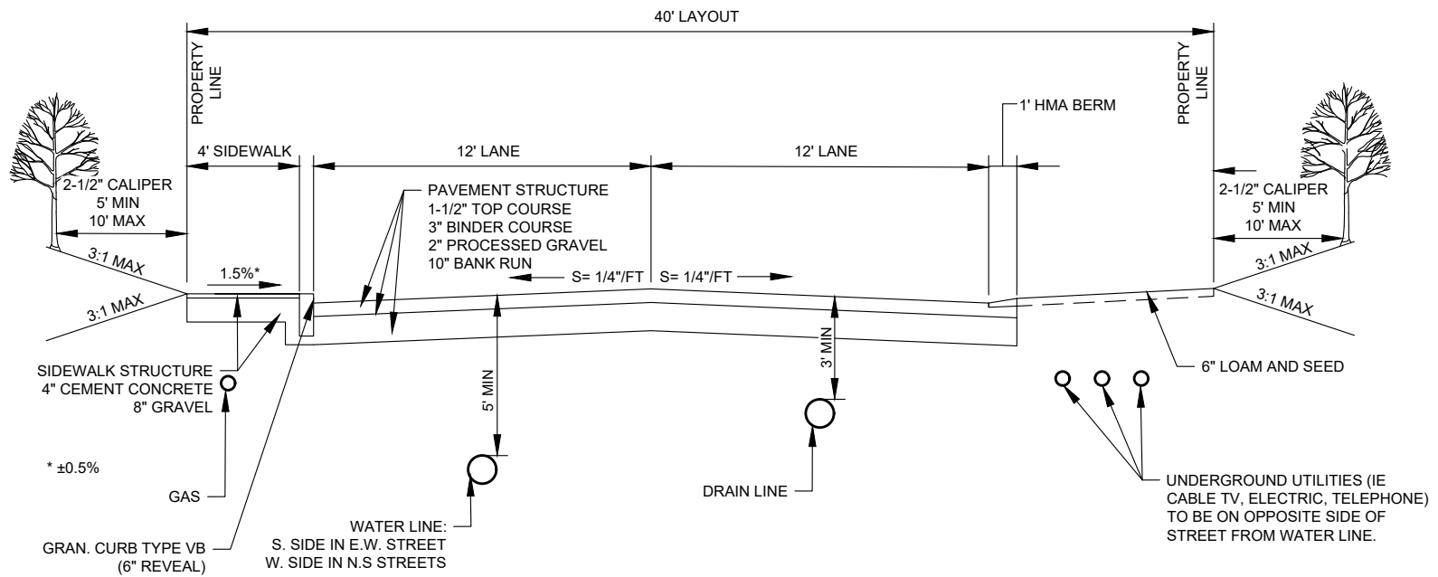
TYPICAL CROSS SECTION - MINOR STREET w/o GRASS STRIP NOT TO SCALE
