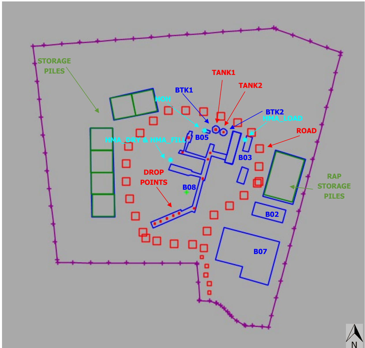
Appendix Figure A-1. Facility Site Layout
