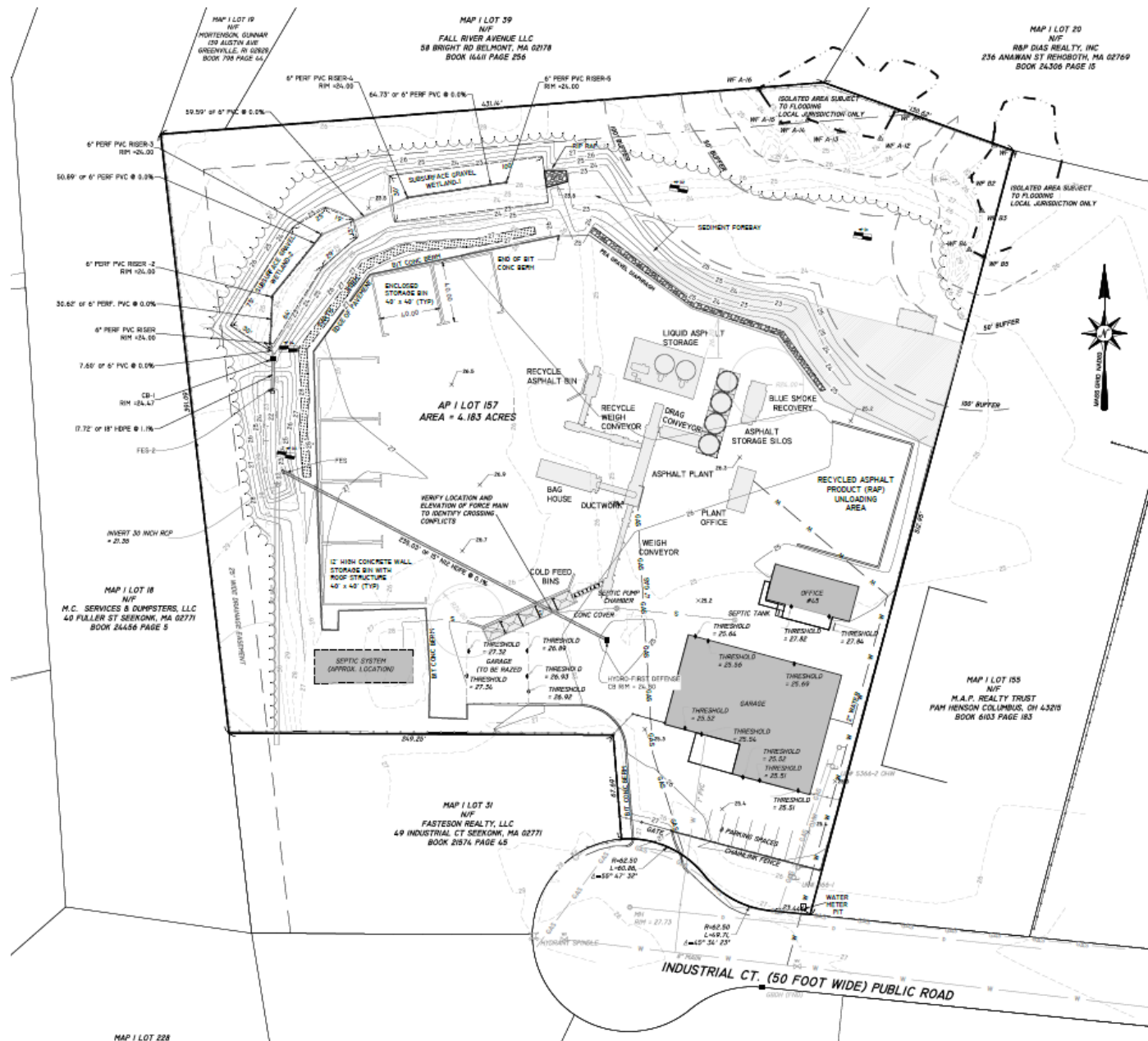
Figure 1-3. Site Layout
